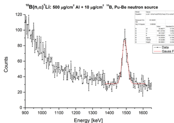
Fig. 3: Spectrum of the ^{10}\text{B}(\text{n},\alpha)^7\text{Li} reaction. The investigated sample is used to calibrate the measurement.
