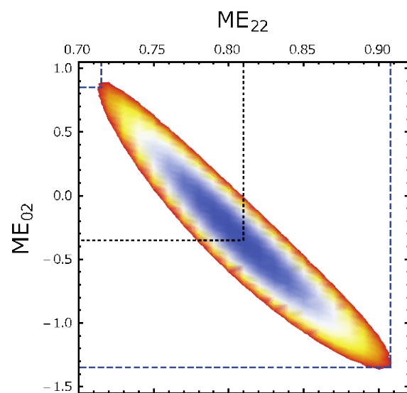
Fig.2: Sum of \chi^2 values resulting from Gosia2 minimisation as a function of the diagonal ( ME_{22} ) and transitional ( ME_{02} ) matrix elements (in eb) for the first 2^+ state in ^{208}\text{Rn} .
