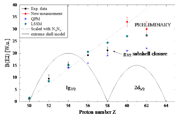
Fig.1: B(E2) in the systematics of the even N=80 isotones from Z=50 (Sn) to Z=64 (Gd). The existing experimental data including our values for ^{140}\text{Nd} [1] and ^{142}\text{Sm} [2] are presented in comparison with theoretical calculations.
