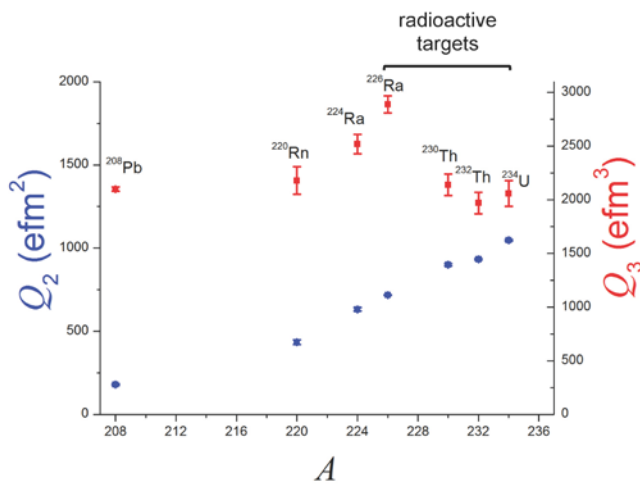
Fig.2: Measured electric-quadrupole and -octupole moments for nuclei in the actinide region. The octupole moment remains almost constant over the mass range, with only ^{224,226}\text{Ra} showing an enhancement.
