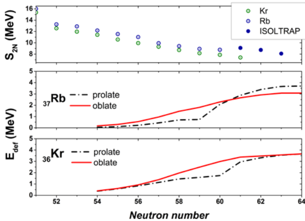
Fig.1: Two-neutron separation energy ( S_{2N} ) for isotopes of Kr and Rb (upper panel) and deformation energy ( E_{\text{def}} ) of the prolate and oblate configurations along the two isotopic chains (middle and lower panel).
