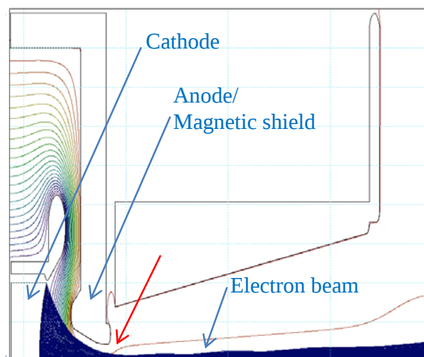
Fig.1: Generation of high compression electron beam in HEC 2 electron gun. The red arrow indicates the injection into a 0.2 T magnetic field which will be gradually increased to 5 T after a short drift region with lower field.
