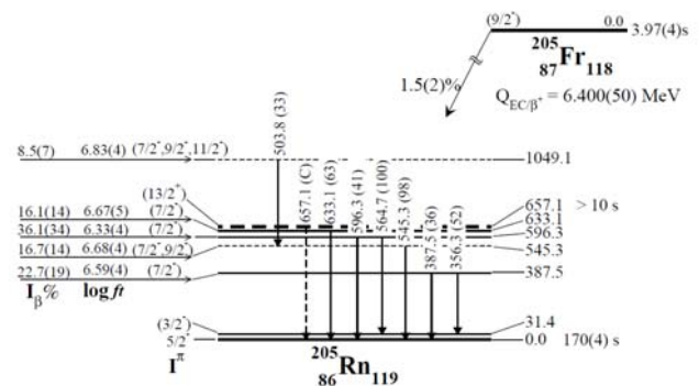
Fig. 2: Level scheme of ^{205}\text{Rn} as obtained from the present work. All the transitions are labeled with their energies and relative \gamma -ray intensities in brackets. Also, all the levels are labeled with their corresponding excitation energies (on the right). "C" indicates that the \gamma -ray transition is highly contaminated (and for the 657.1 keV transition the placement is based on K-shell conversion electrons).
